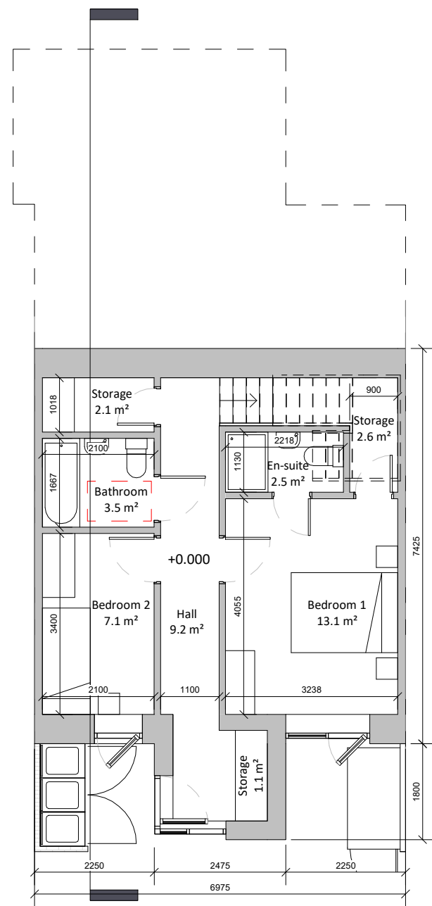
1 Ground Floor Plan (Duplex 3A) 1 : 100
