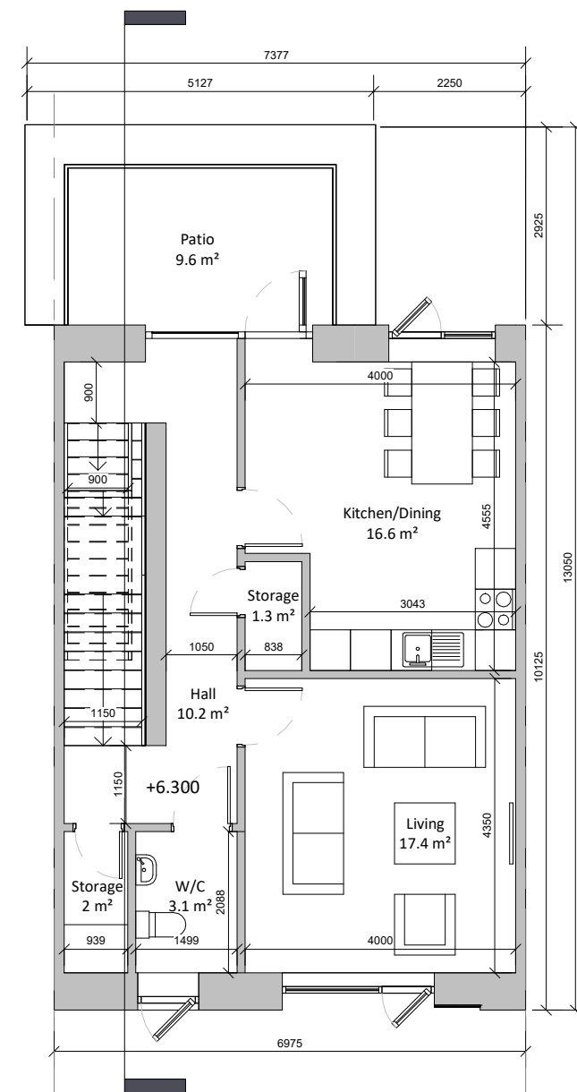
3 Second Floor Plan (Duplex 3B) 1 : 100
