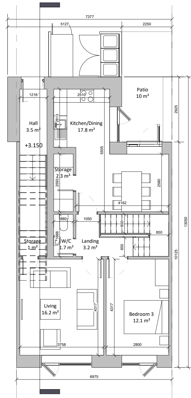
2 First Floor Plan (Duplex 3A & 3B) 1 : 100
