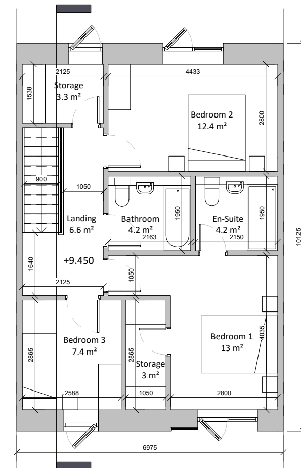
4 Third Floor Plan (Duplex 3B) 1 : 100
